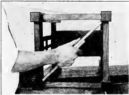
FIG. 421-a. TESTING FRAME FOR SQUARENESS BY MEASURING DIAGONALS.
